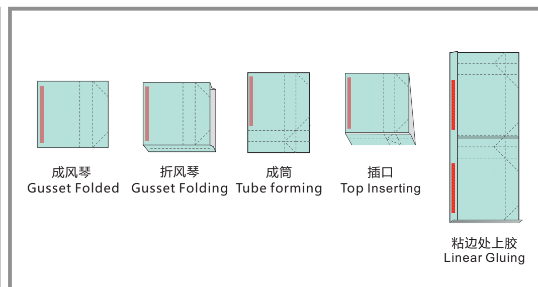
糊筒部套 ( LxW) Tube Forming 6.0x1.4M
